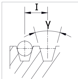
V grooves without undercut
