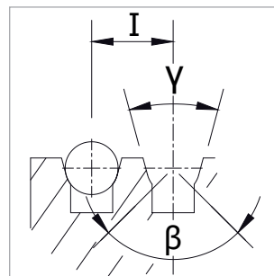
U grooves with undercut
