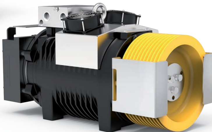
SG38F Gearless with fan kit
