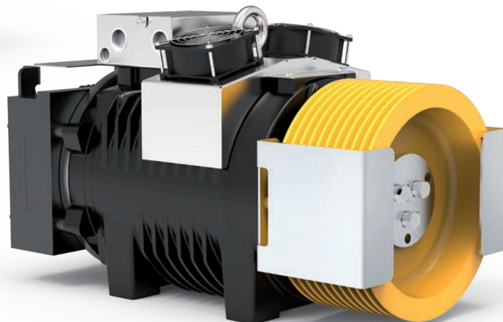
SG30F Gearless with fan kit
