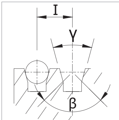
V grooves with undercut
