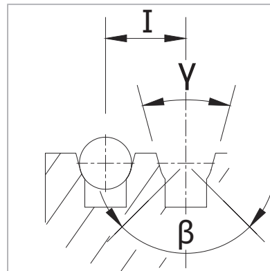
U grooves with undercut
