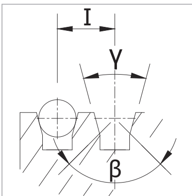
V grooves with undercut
